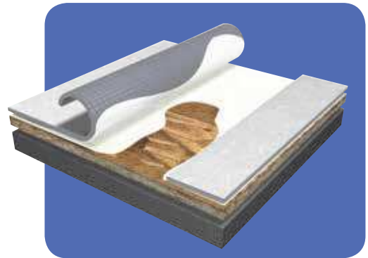
PVC Fully Adhered with WBBA 2000 Contact Bonding Adhesive
