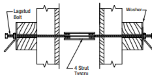
4-Strut
