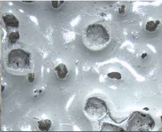
Traditional Aggregate Controlled abrasion test: notice "Pop Out" of aggregate
