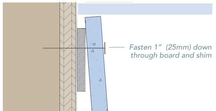
Top/Terminal Course Fastening
