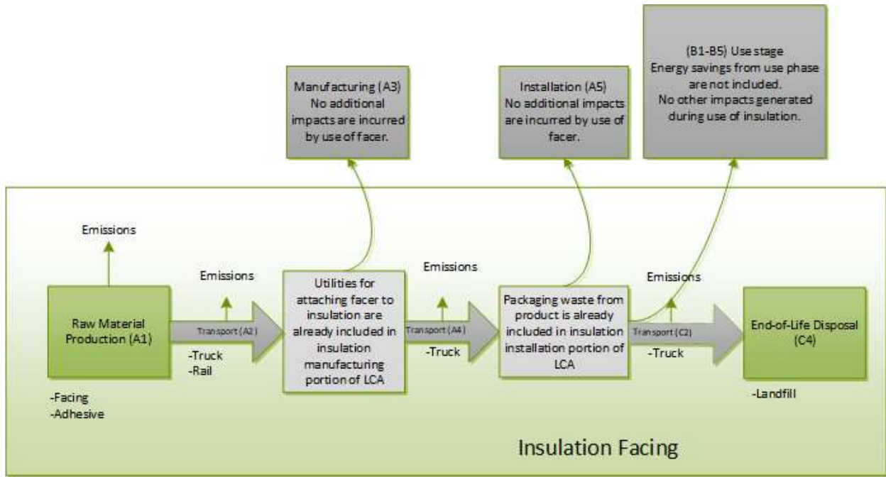
Figure 2. Flow diagram/System Boundary for Insulation Facing
