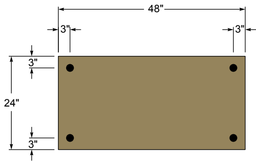
24 in. x 48 in. Panel with 4 Fasteners
