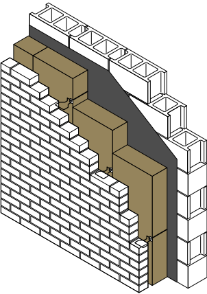
Masonry Ties
