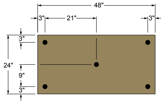
24 in. x 48 in. Panel with 5 Fasteners
