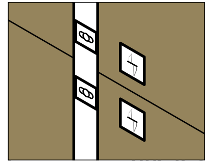
Post insulation installation
