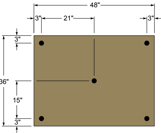
36 in. x 48 in. Panel with 5 Fasteners
