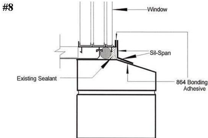
Picture#8:Pre-formed Joint Sealant
