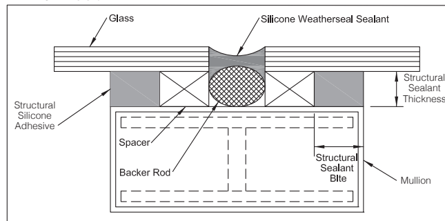
TYPICAL SSG DETAIL
