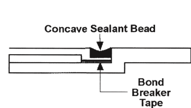
Recommended Joint Design With Bondbreaker Tape
