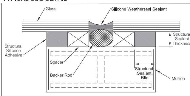
TYPICAL SSG DETAIL
