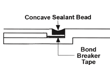
Recommended Joint Design With Bondbreaker Tape
