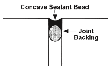
Recommended Joint Design With Joint Backing
