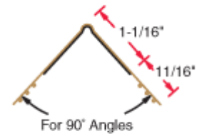
For 90° Angles Drawing not to scale
