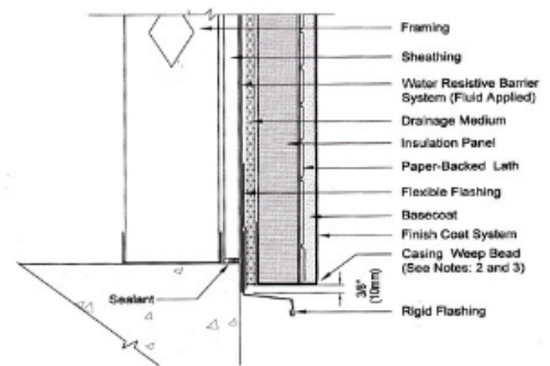
Stucco Base of Wall Detail
