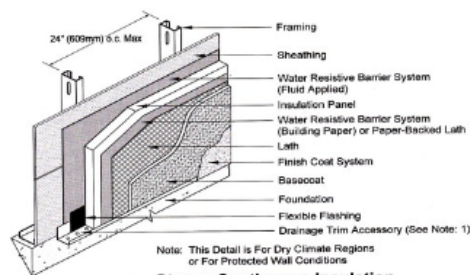
Stucco Continuous Insulation
