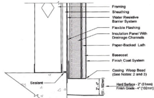
Stucco Base of Wall Detail
