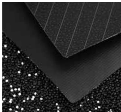
DURA♦SKRIM® J & N-SERIES REINFORCED " TEXTURED LLDPE
