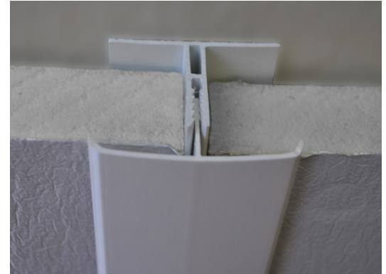
Flex-Tite Insulation Attachment System
