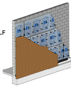
Concrete-CMU Brick Cladding R-SEAL 2000 LF
