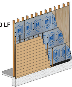
Wood Stud Fiber-Cement Lap Siding R-SEAL 2000 LF
