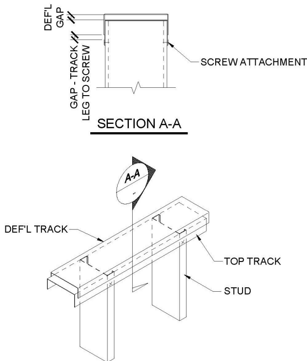
Figure 3: Light-gauge Steel Framing Movement Joint (from Steel Stud Manufacturer's Association, pg. 30)
