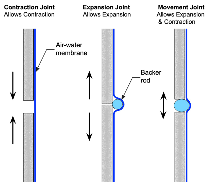
Figure 5: Three categories of joints
