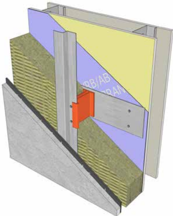
Example of the use of galvanized sheet steel strips to provide structural backer for cladding support clips away from studs.
