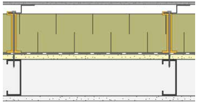
Uninsulated 3 5/8" steel stud wall with exterior insulation and cladding attachment system.
