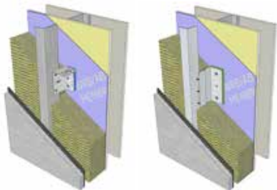
Thermally isolated galvanized steel clip attached to wall with screws through plastic isolation pad.
