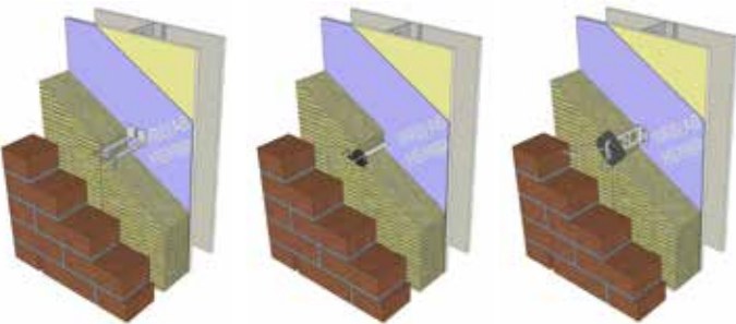
Examples of alternate masonry ties installed through ROCKWOOL CAVITYROCK® insulation.
