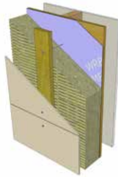
Long screws through vertical wood strapping and rigid ROCKWOOL COMFORTBOARD™ insulation on a multi-family residential project.
