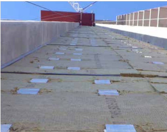
Example of insulation retained by intermittent cladding support clips behind metal panels. The metal panel support structure overtop will further retain the insulation in the assembly here.
