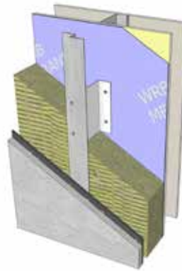
Intermittent stainless steel clips with vertical girts.
