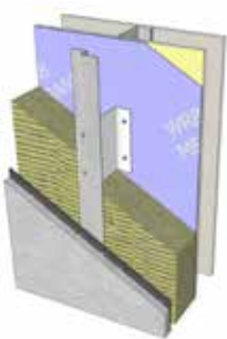
Intermittent galvanized steel clips with vertical girts.
