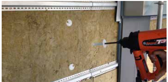
Example of plastic fuel-cell actuated insulation fasteners installed after insulation and girt system is installed to retain the insulation.
