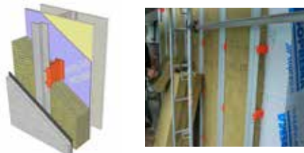
Fiberglass clips with vertical Z-girt attached with screw fasteners through the fiberglass clips into the back-up wall.
