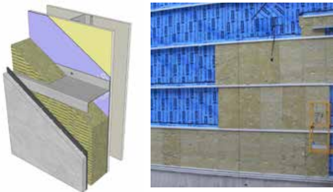
Horizontal Z-girts over a steel stud wall assembly. Girts are fastened every 36" here to reduce the thermal bridging.
