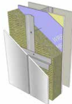
Long screws through horizontal metal hat tracks and rigid ROCKWOOL COMFORTBOARD™ insulation on a commercial building project.
