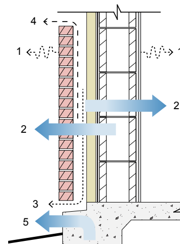
Figure 4b: Dry Mechanism for Walls
