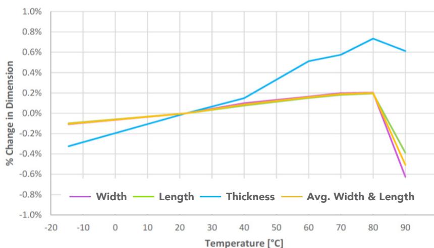
Figure 3 Summary of Average Insulation Dimensional Changes for EPS
