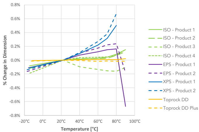
Figure 7 Average Length and Width Dimensional Changes for all Tested Products
