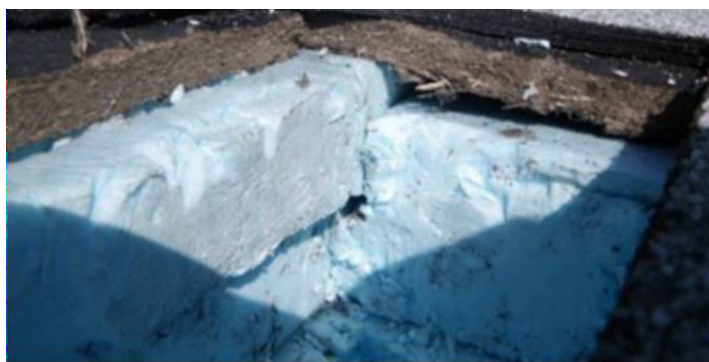
Figure 1 Irreversible thermal expansion of XPS within a conventional roof assembly potentially due to high in-service temperature.
