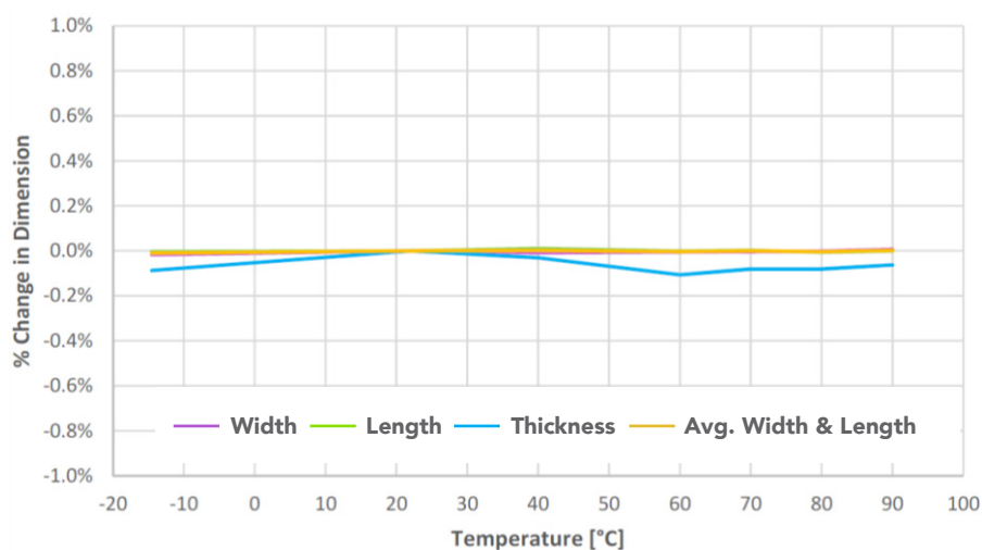
Figure 6 Summary of Average Insulation Dimensional Changes for Stone Wool
