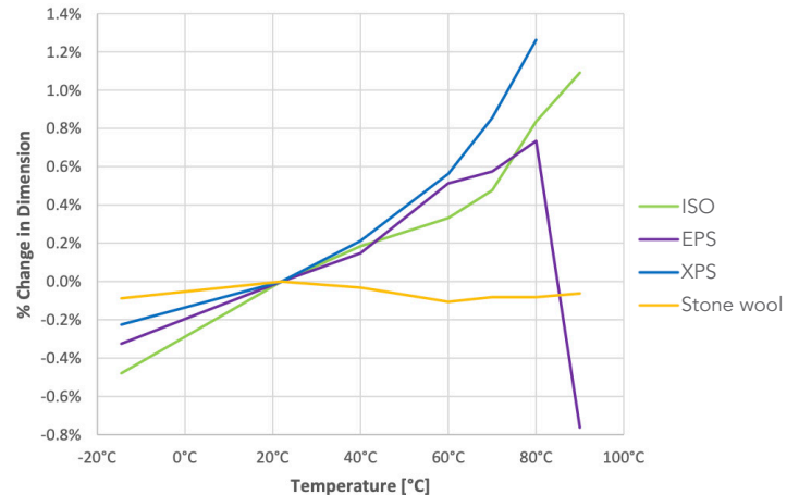
Figure 10 Average Thickness Dimensional Changes for each Insulation Type
