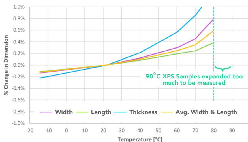
Figure 4 Summary of Average Insulation Dimensional Changes for XPS
