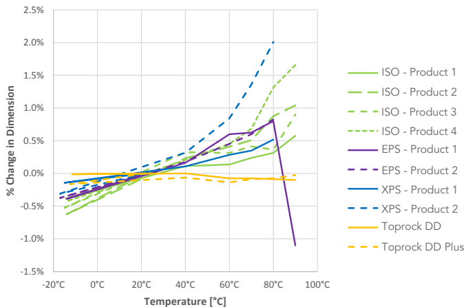
Figure 8 Average Thickness Dimensional Changes for all Tested Products
