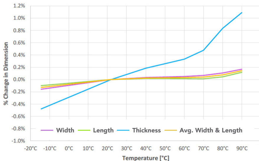
Figure 5 Summary of Average Insulation Dimensional Changes for ISO
