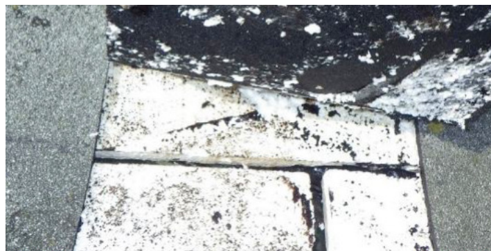
Figure 2 Permanent shrinkage of EPS insulation in a conventional roof assembly, potentially due to high in-service temperature or initial application into hot asphalt adhesive.
