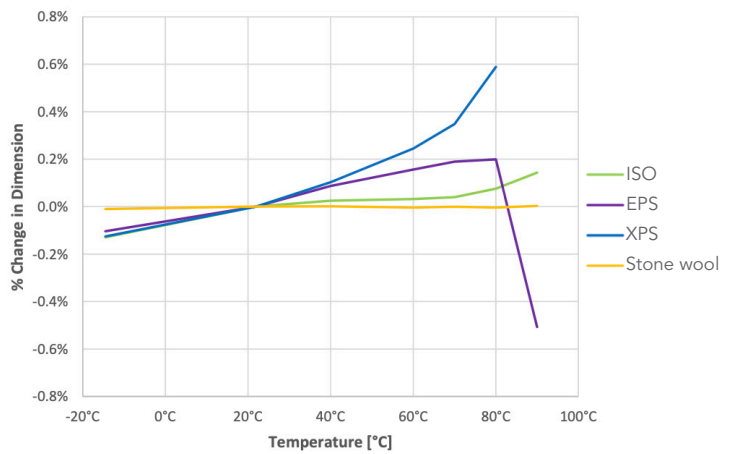
Figure 9 Average Length and Width Dimensional Changes for each Insulation Type
