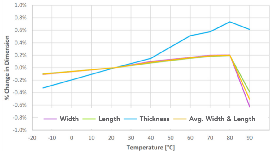
Figure 3 Summary of Average Insulation Dimensional Changes for EPS
