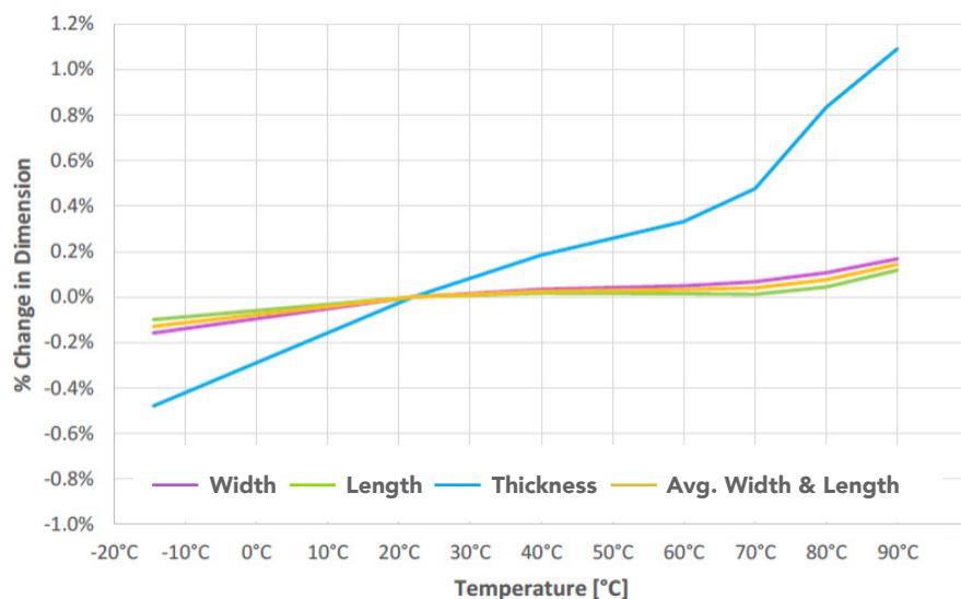
Figure 5 Summary of Average Insulation Dimensional Changes for ISO
