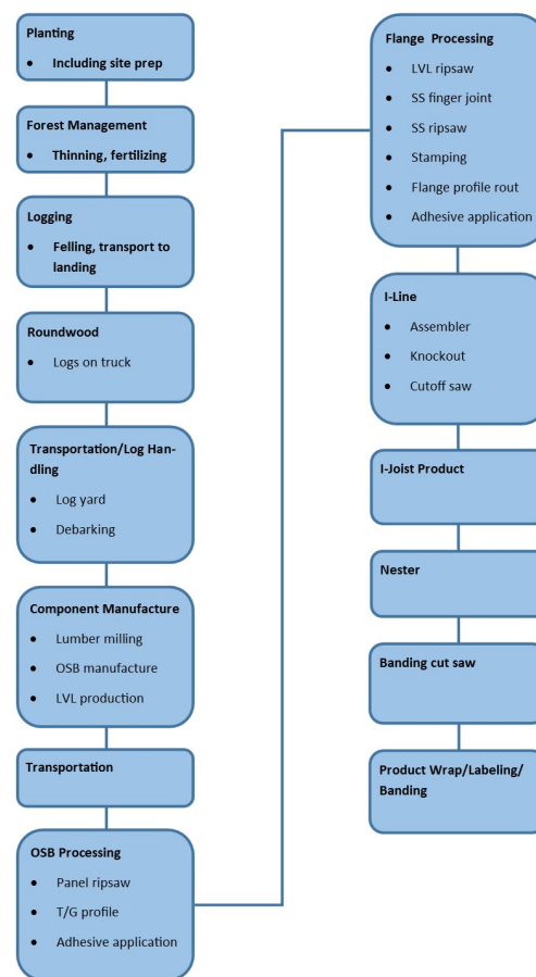
Figure 1: Cradle-to-gate product system for I-joist
