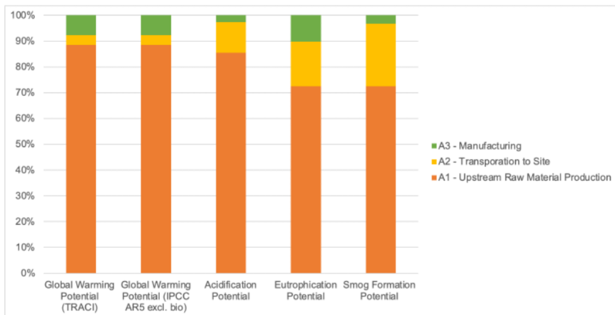
Figure 3 : Dominance analysis for 1 linear meter of I-joist produced by Roseburg (weighted average).
