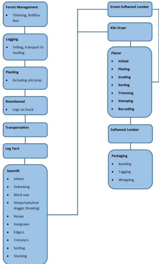
Figure 1: Cradle-to-gate product system for kiln-dried, planed softwood lumber
