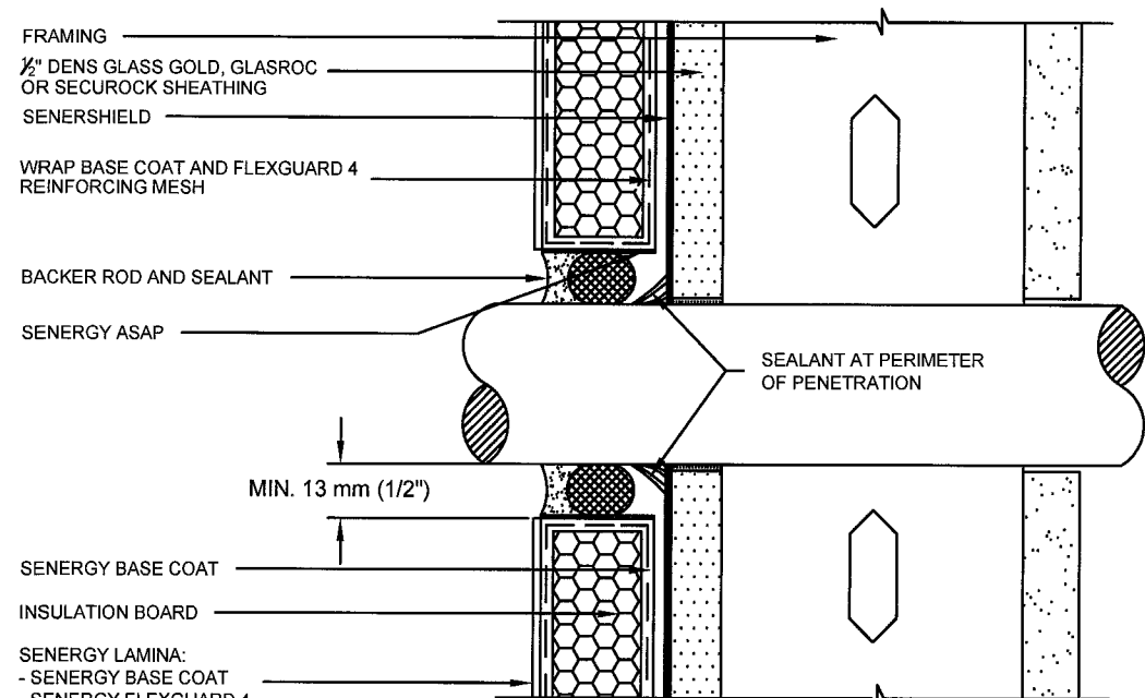
PIPE PENETRATION
