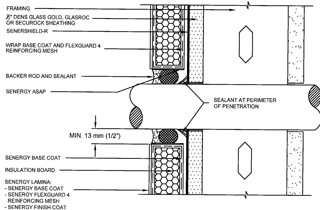
PIPE PENETRATION
