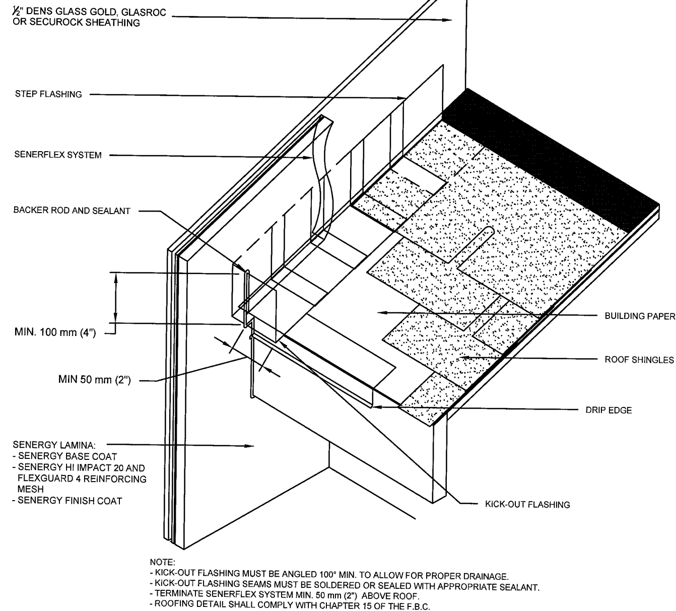
KICK-OUT FLASHING DETAIL
