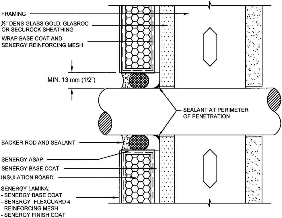
PIPE PENETRATION
