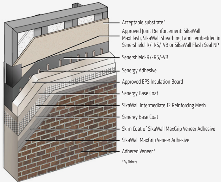
SenerPanel Channeled Adhesive CI Design with SikaWall-1000 MaxGrip Veneer Adhesive
