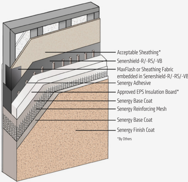
SenerPanel Channeled Adhesive CI Design
