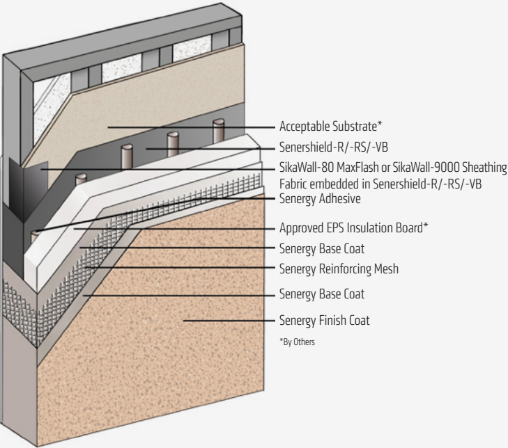
SenerPanel Secondary Weather Barrier
