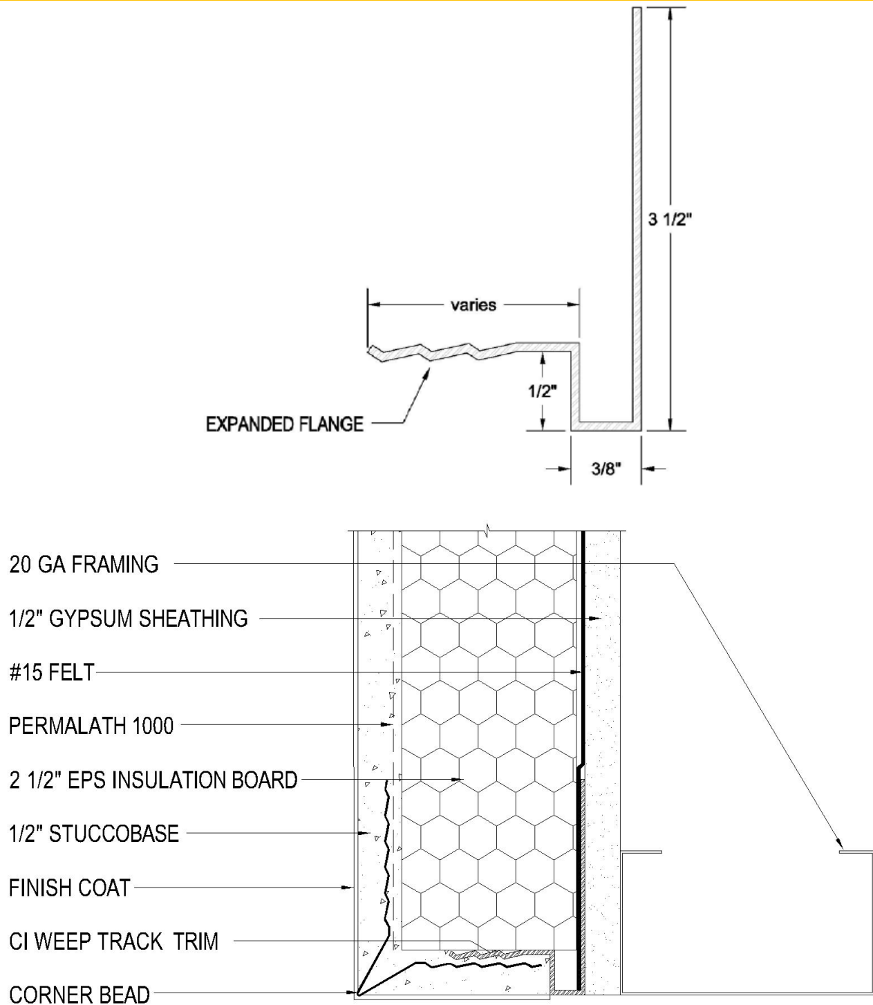
Figure 1 – Typical opening detail for NFPA 285 assembly (See Table 5)
