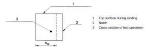
Figure 39 : Position of the notch in an EN14651 beam
