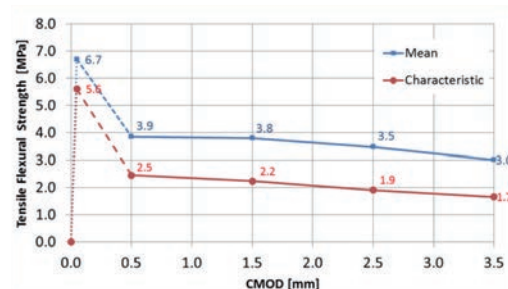
Figure 9 : Results from EN14651 tests for steel fibre reinforced concrete segments from a London project
