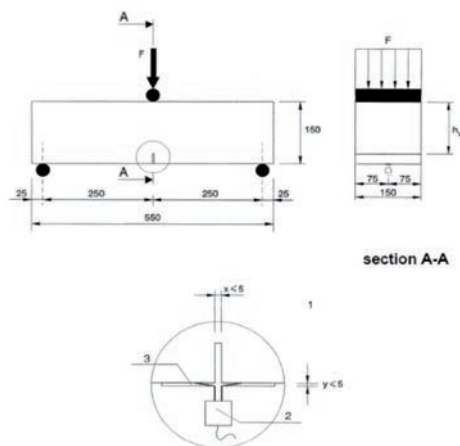
Figure 40 : EN14651 test setup with CMOD transducer
