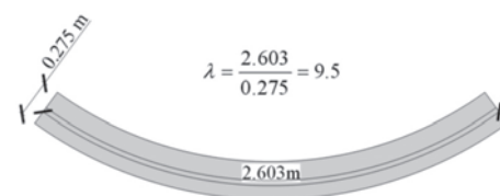
Figure 2 : An example of a segment aspect ratio \lambda .
