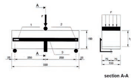
Figure 41 : EN 14651 test setup with deflection transducer
