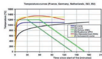
Figure 35 : Fire time-temperature curves (ITA 2004)
