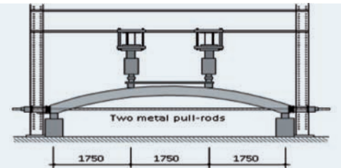
Figure 20 : Flexural tests on tunnel segment
