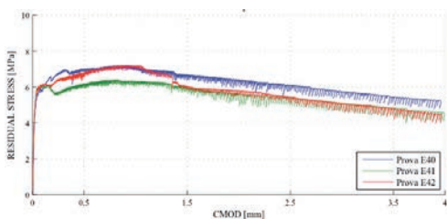
Figure 10 : Typical test data for a C35/45 4.0c concrete
