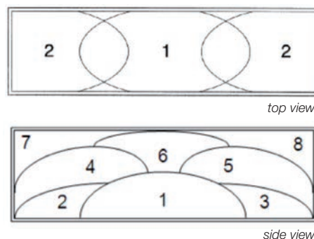
Figure 38 : Alternative method to fill moulds for EN14651 beams
