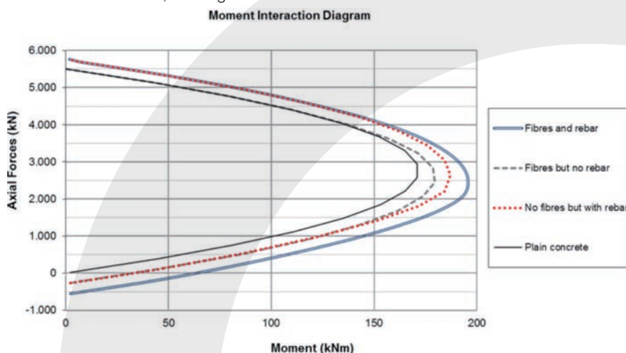
Figure 3 : Moment – Axial thrust interaction diagram showing various forms of reinforcement (for 250 mm of C40/50 5c concrete with 8/8 mm 150/150 mm c/c mesh) 3
