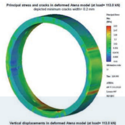
Figure 30 : Finite element analysis designs by JKP Static
