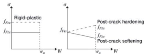
Figure 11: Simplified post-cracking constitutive laws: stress-crack opening (continuous and dashed lines refer to softening and hardening post-cracking behaviour respectively)
