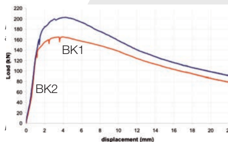
Figure 16 : Bending tests: load-displacement diagrams
