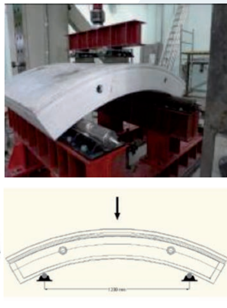
Figure 15 : Bending test set-up
