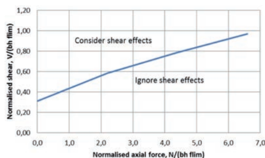
Figure 4 : Simplified shear check after Coccia et al (2015). Where V is the shear force, N is the axial force, b is breadth, h is depth and f_{lim} is the design tensile strength.
