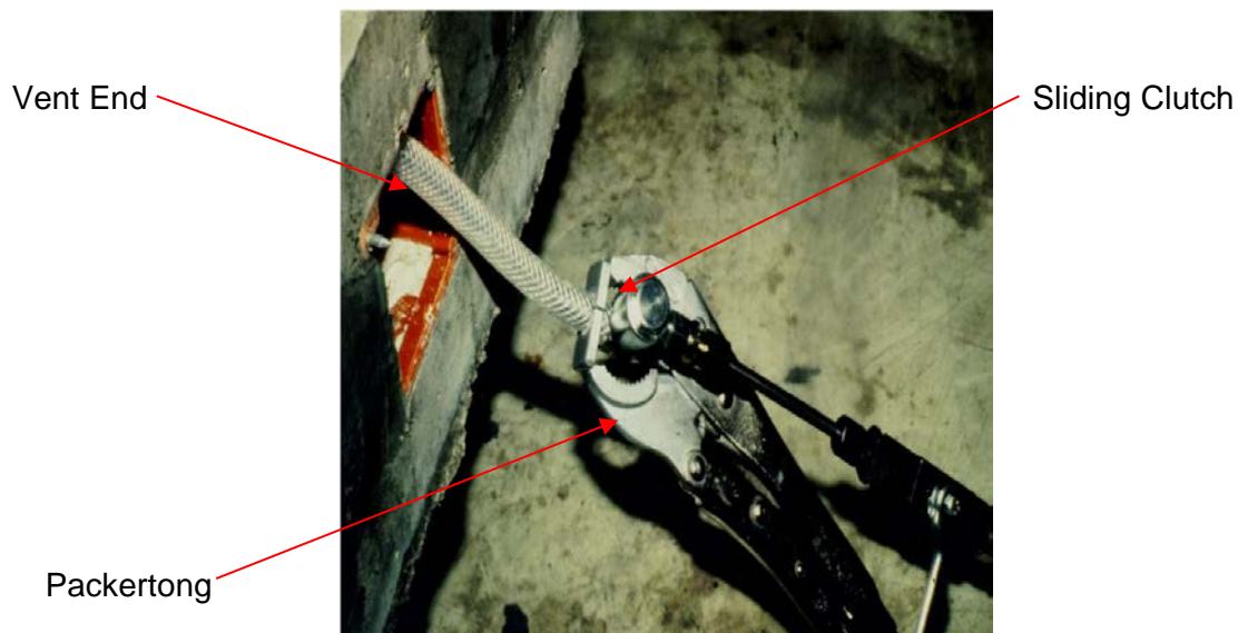
Figure 3: Injection Equipment Assembly
