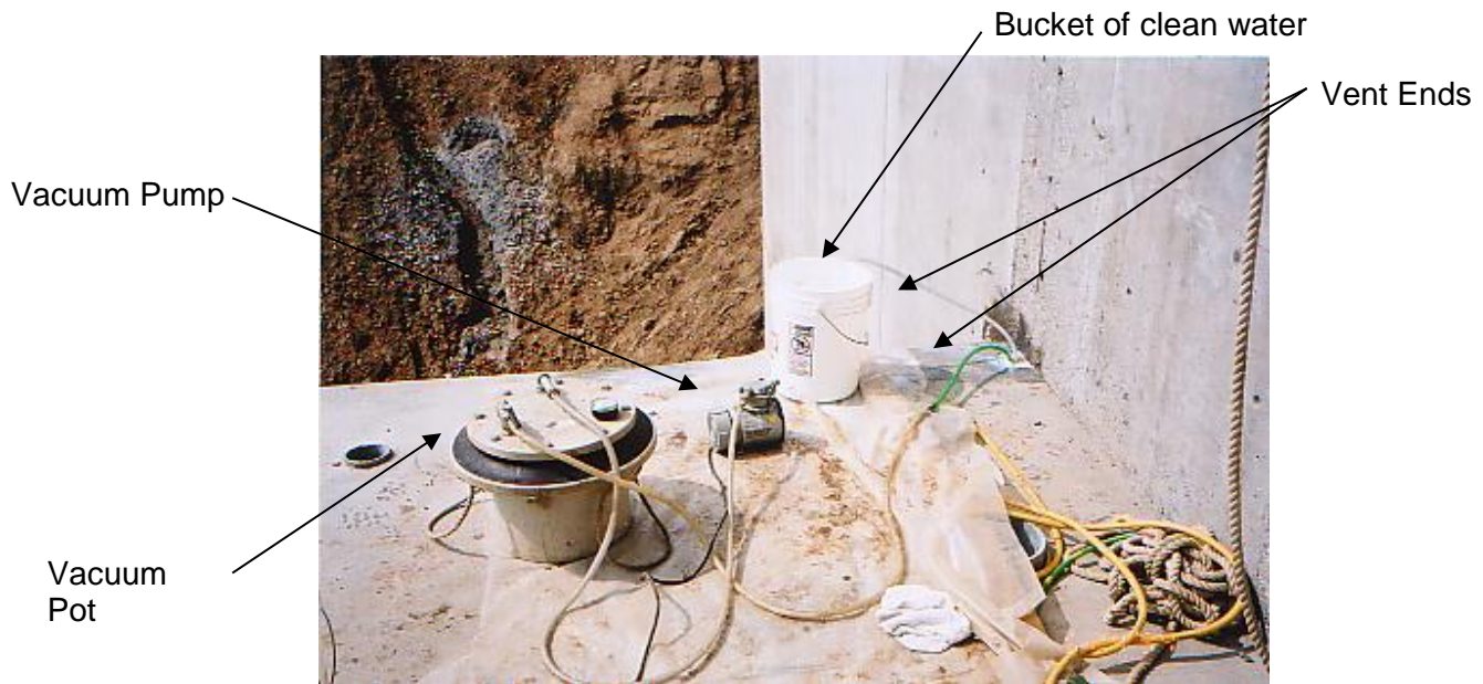
Figure 4: FUKO Hose Cleanout Overview
