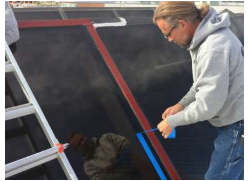
Always pull the tape while the Sikalastic® Clearglaze is wet to leave a clean sharp edge.
