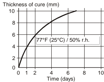
Diagram 1: Curing speed Sikasil® SG-15
