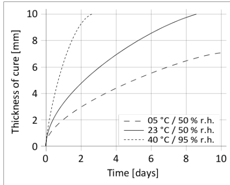
Diagram 1: Curing Speed of Sikasil® WS-305 AM
