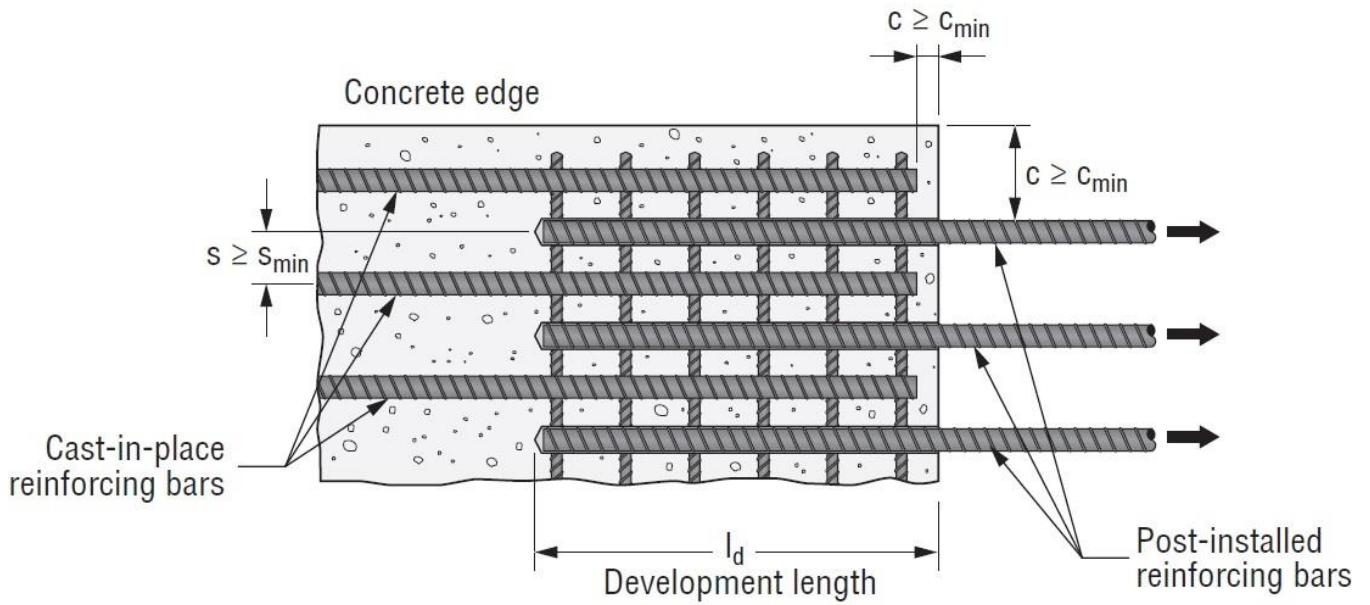
FIGURE 1—INSTALLATION PARAMATERS FOR POST-INSTALLED REINFORCING BAR CONNECTIONS
