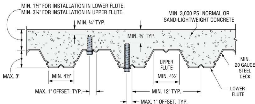
FIGURE 3—INSTALLATION OF \frac{3}{8} -INCH AND \frac{1}{2} -INCH SHANK DIAMETER SCREW ANCHORS AND ROD HANGERS INTO THE SOFFIT OF CONCRETE-FILLED PROFILE STEEL DECK FLOOR AND ROOF ASSEMBLIES (1 in = 25.4 mm)
