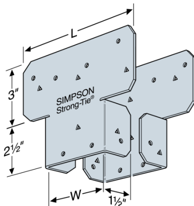
FIGURE 3a—AC POST CAP CONNECTOR COMPONENTS
