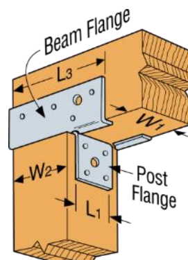
Typical EPC End Post Cap Installation
