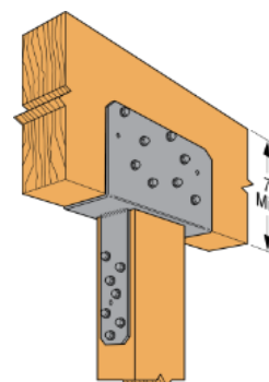
CCQ46SDS2.5 Installation
