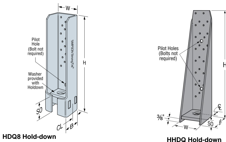
FIGURE 2A—HDQ8/HHDQ SERIES HOLD-DOWNS
