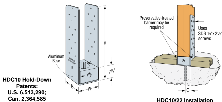
FIGURE 4—HDC10 HOLD-DOWN
