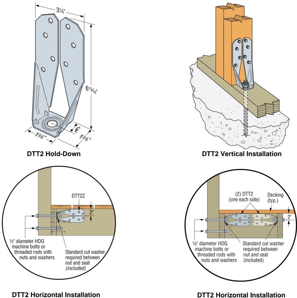
FIGURE 3—DTT2 HOLD-DOWN
