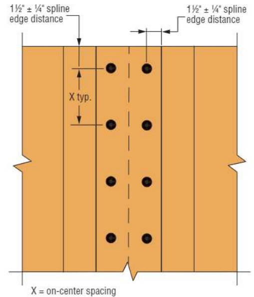
Figure 2: Fastener layout plan — Fastener end distance in the spline shall be 1.5 ± 0.25", and fastener edge distance in the spline shall be 1.5 ± 0.25". The nominal fastener spacing is "X".
