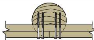
Notched, Lap
