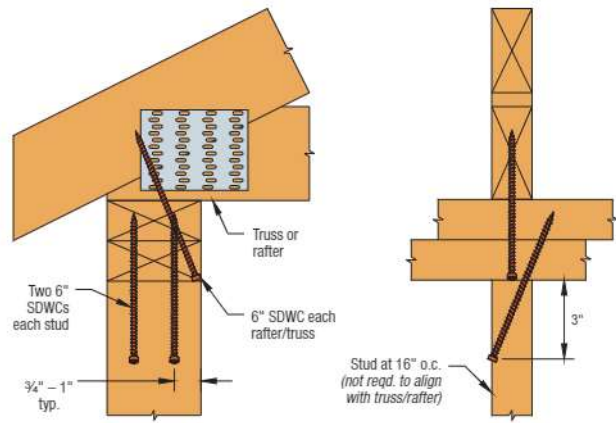
Wall Assembly B Two SDWC as Angled Stud Screw
