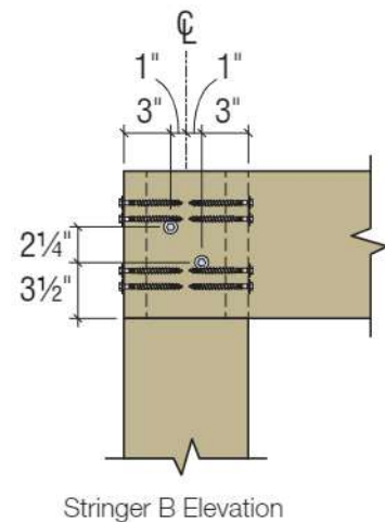
Detail SC1 — 8" Square Pile
