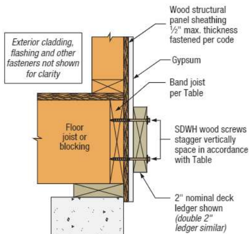
Ledger-to-Rim Board Assembly (wood-framed lower floor acceptable, concrete wall shown for illustration purposes)
