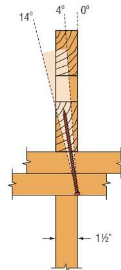
Installation Angle Limit (front view)
