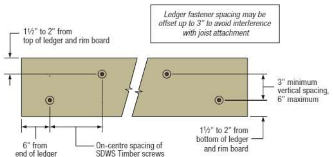
SDWS Timber Screw Spacing Detail for Ledgers
