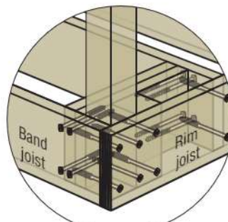
Detail B Isometric View
