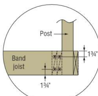
Detail B.2 Side Elevation
