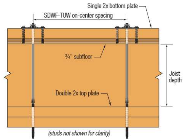
SDWF-TUW Assembly
