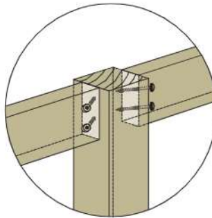
Detail A: Rail-to-Post Perspective View
