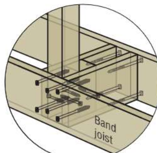
Detail A Isometric View
