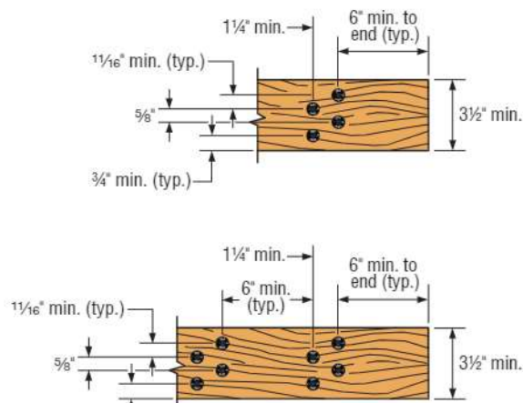
Spacing Details
