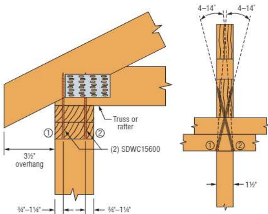
Configuration A: Truss Aligned with Stud Install Through Top Plate into Rafter/Truss
