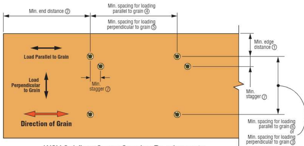
WSV Subfloor Screw Spacing Requirements
