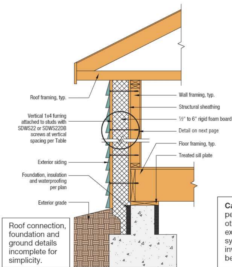
Wall Cross-Section
