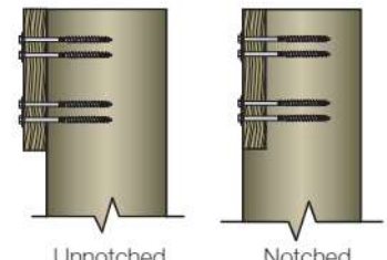
Section View
