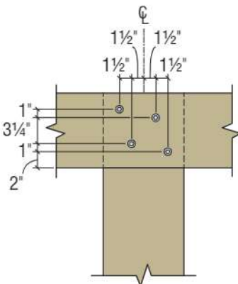
Detail SQ2
