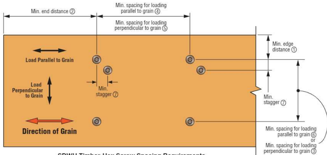
SDWH Timber-Hex Screw Spacing Requirements
