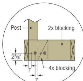
Detail A.2 Side Elevation
