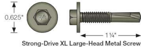
Strong-Drive XL Large-Head Metal Screw
