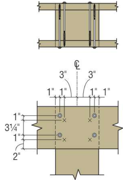
Detail SQ5 — 12" Square Pile Two-Sided 2x10
