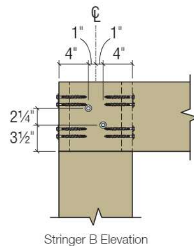
Detail SC2 — 10" Square Pile
