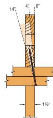
Allowable Installation Range (front view)
