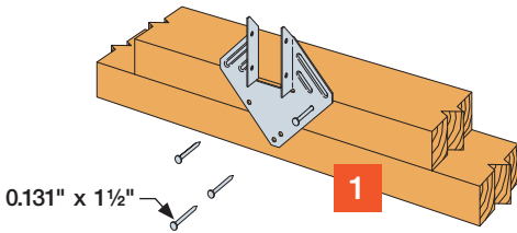
Truss and Plates Cercha y placas
