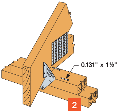
Truss and Plates Cercha y placas
