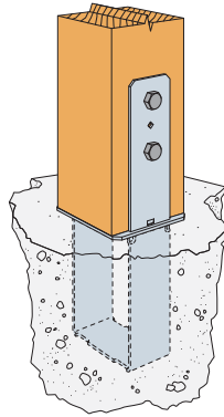
Similar CB Installation (typ.)
