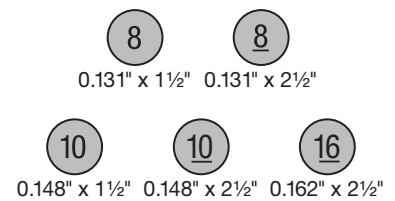
SCN Smooth-Shank Head Stamps
