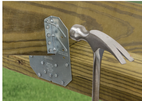
Strong-Drive SCN Smooth-Shank Connector Nail
