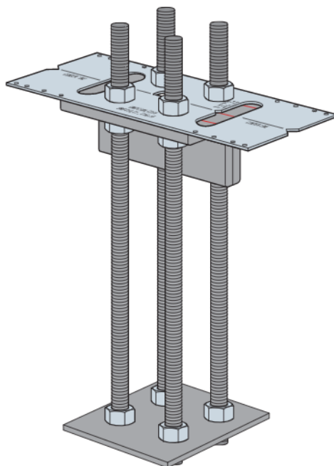
MFSL Anchorage Assembly US Patent 8,336,267
