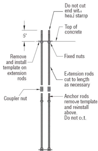
MFAB Anchorage Assembly with Extension Kit
