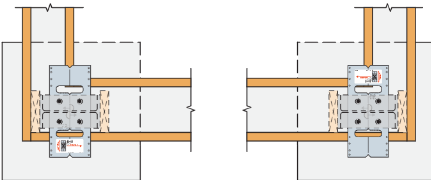
Top view of frame opening showing correct orientation of MFSL template
