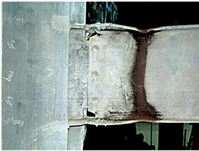
Figure 1 — Formation of Plastic Hinge at RBS Connection (Reference: Gilton, Chi and Uang, UCSD SSRP-2000/03)
