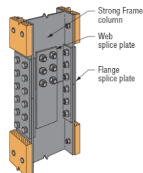
Figure 4 -- Spliced-Column Design Option
