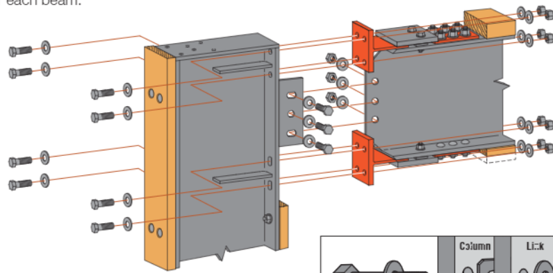
T-Stub Yield-Link
