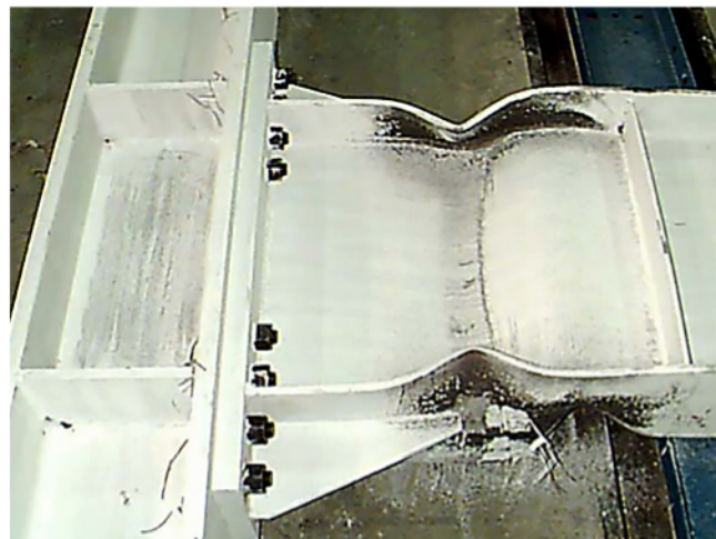
Figure 3 — End Plate Specimen at Failure (Reference: Sumner et al. 2000)
