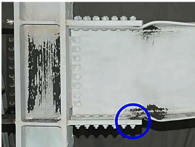
Figure 2 — Fracture of Beam Flange Plate Moment Connection (Reference: Sato, Newell and Uang, UCSD SSRF -2007)
