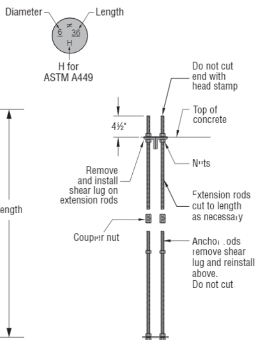
MFSL Anchorage Assembly with Extension Kit US Patent 6,336,267 B2
