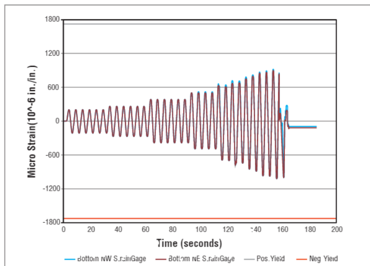
Figure D4a.3 — Measured Strain from Testing at Beam Bottom Flange
