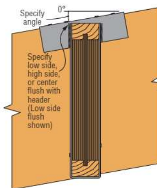
Typical WP Top Flange Sloped Down Left with Low Side Flush
