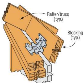
Typical RBC Installation Over 1" Foam Board®
