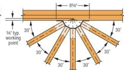
THJM2-5-SDS3 Top View Installation
