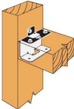
Typical APRTR Installation
