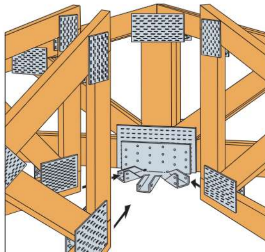
Typical LTHMA Installation (terminal hip truss condition)
