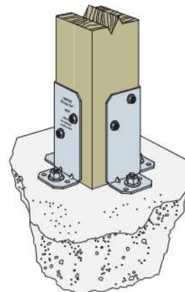
RPBZ Installation in Exterior Environment
