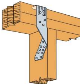
Typical TSP Installed to Top Plate
