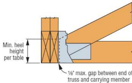
HTU Installation for Standard Allowable Loads (for ⅛" maximum gap, use Alternate Allowable Loads.)
