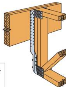
THA422 Face-Mount (Min.) Installation
