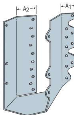
HSULC Available for 3" - and 3 1/2" -wide joists only
