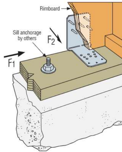
Typical FWANZ Installation
