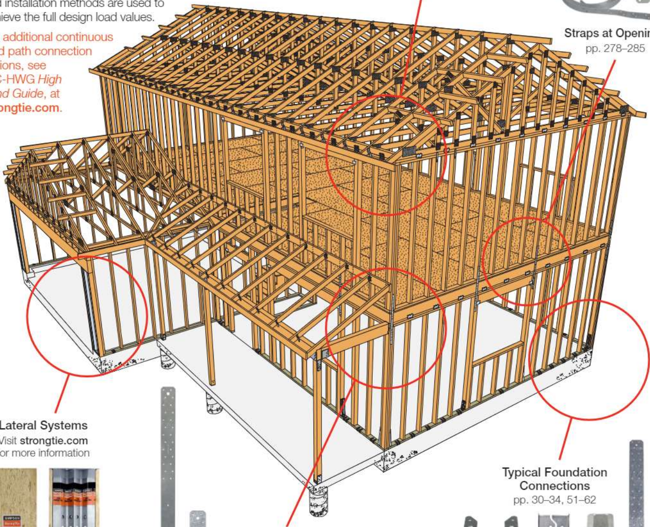
Typical Floor-to-Floor Connections
