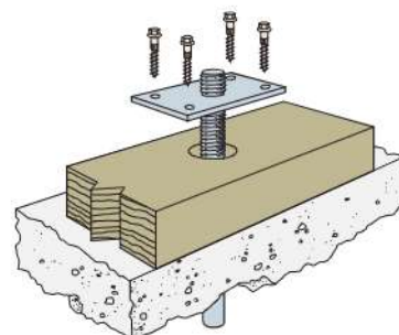
The BP5/8SKT is used when 5/8 inch diameter sill bolt holes are overdrilled
