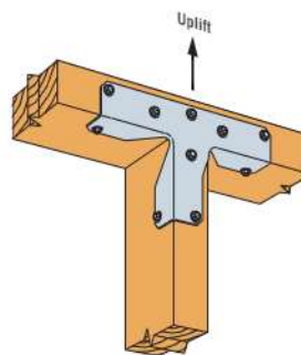
RTT22Z Installation
