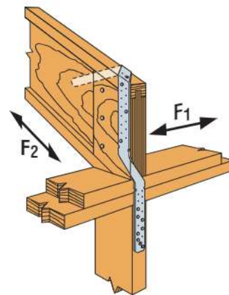
MTS30 Installation with I-Joist Rafter
