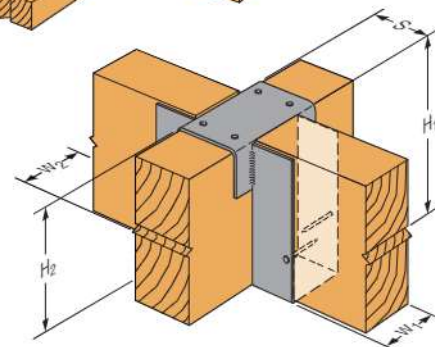
Typical WPD Saddle Hanger Installation
