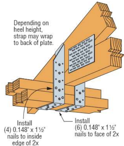
H16 Installation
