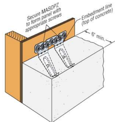
Typical MASOPZ Installation in Concrete
