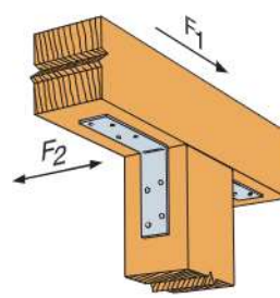
A44 Installation (A33 similar)
