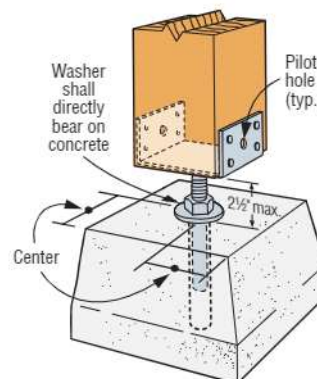
Typical EPB44PHDG Pier Block Installation (supported by a nut)
