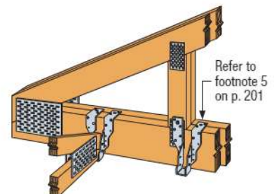
Typical THA29 Top Flange Installation
