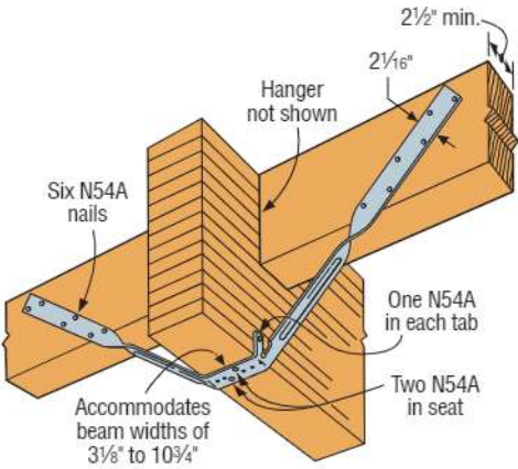
Typical VB Installation
