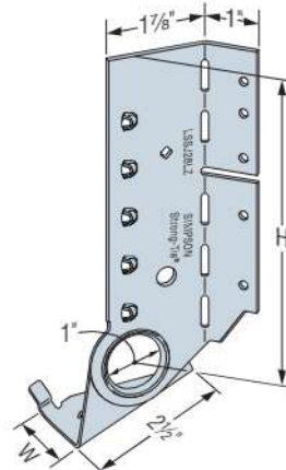
LSSJ28LZ (others similar) US Patent Pending
