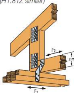
6 H2.5T Installation
