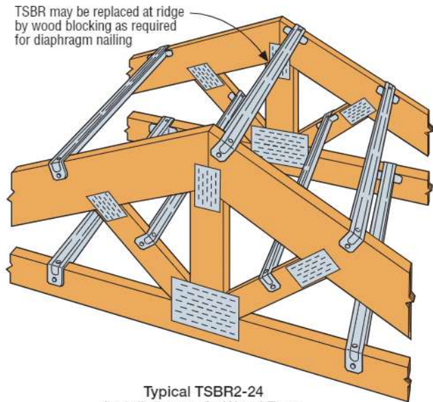
Typical TSBR2-24 Installation on 2x Wood Truss
