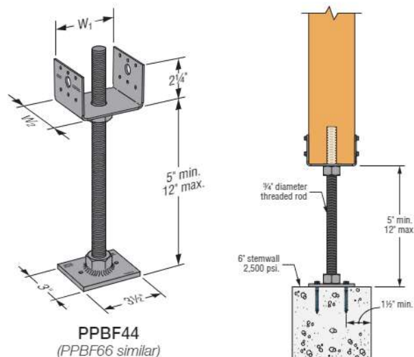
Typical PPBF Installation (before slab pour)
