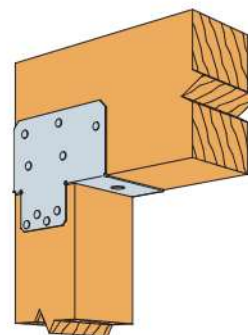
Typical EPCZ End Post Cap Installation
