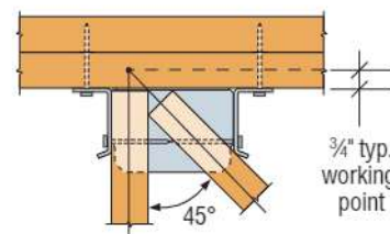
THJU26 Top View Right-Hand Hip Installation
