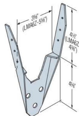
LMA4Z (LMA6Z similar)
