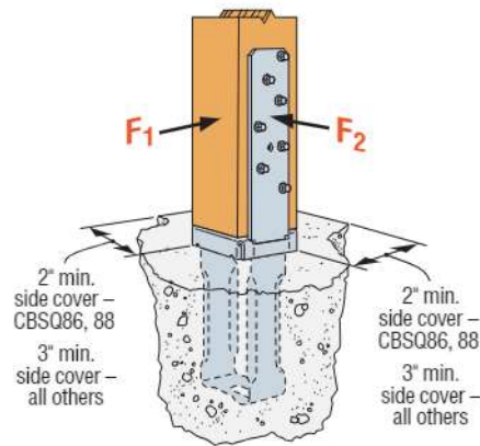
Typical CBSQ-SDS2 Installation
