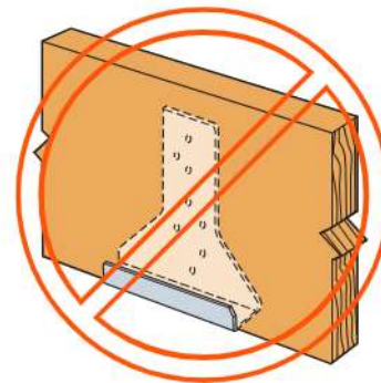
Misinstallation
