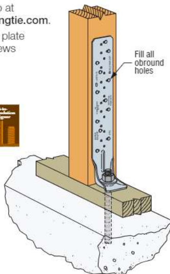
Typical LTPP2 Installation for Holddown Application
