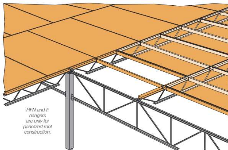
Typical Hybrid Panelized Roof System
