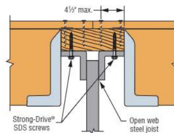
Double HF26N Nailer Installation on Hybrid Truss
