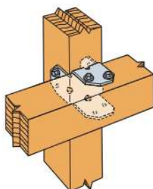
RTB22 Installation
