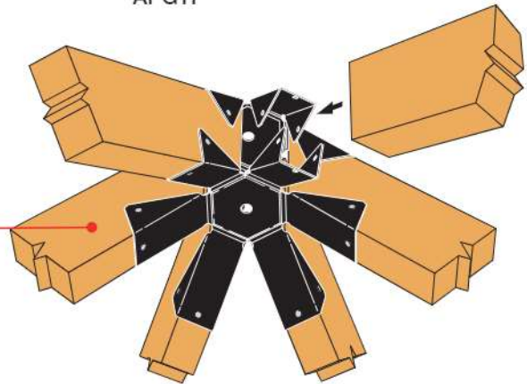
Typical APTG6 Installation
