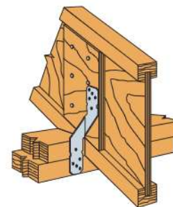
13 H8 attaching I-Joist to Double Top Plates
