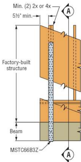
MSTC66B3Z Installation
