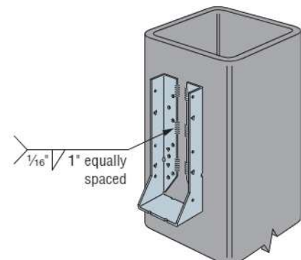
HUC Welded to Steel Column (HUCQ similar)
