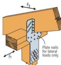
16 H10S Installation
