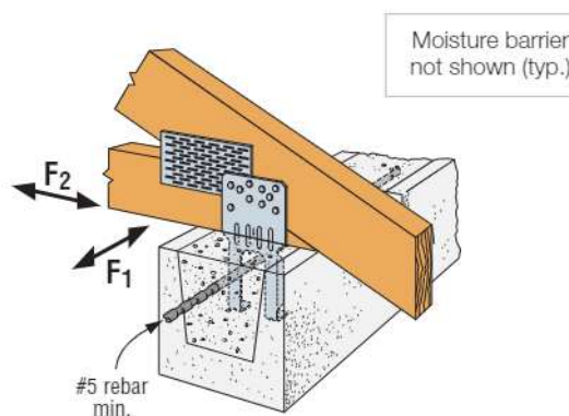
LTA2 Perpendicular-to-Wall Installation
