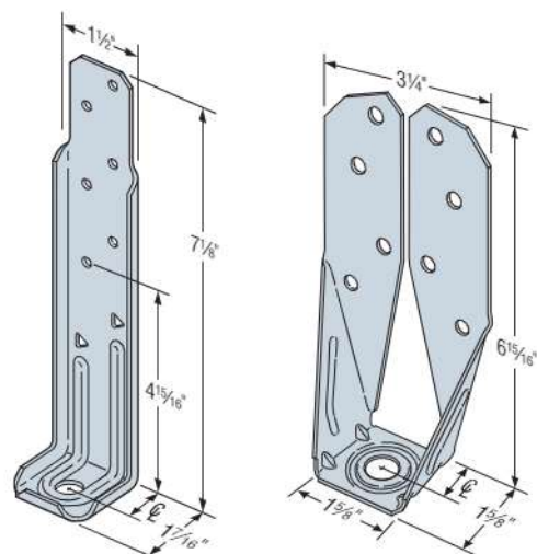
DTT1Z US Patent 10,865,558
