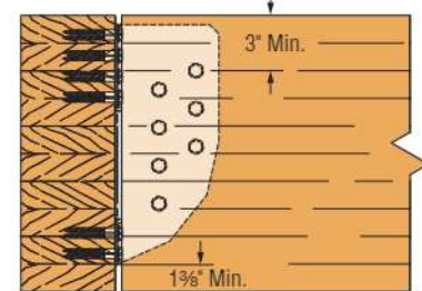
Typical HCJTZ Installation
