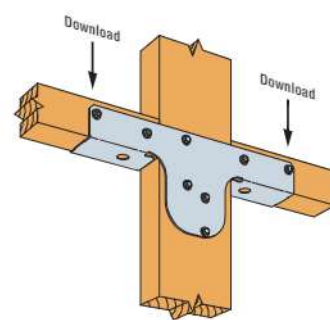
RTF2Z Installation
