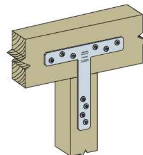
Typical 1616HTQ Installation
