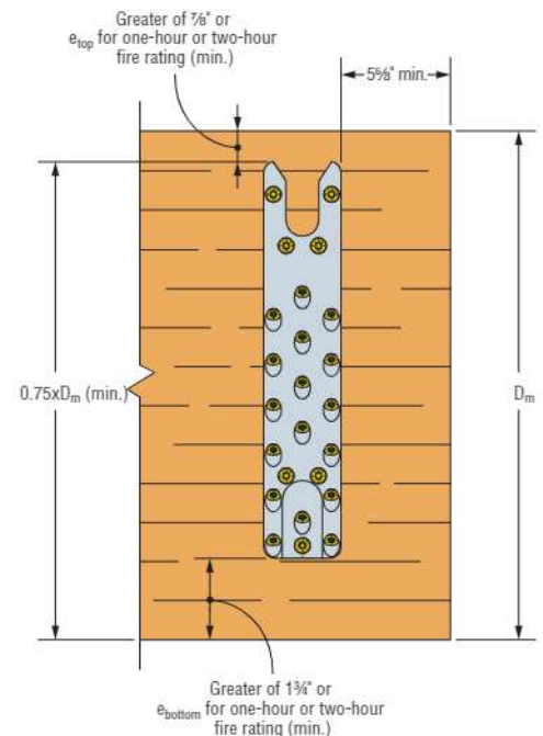
Single ACBH on Carrying Beam
