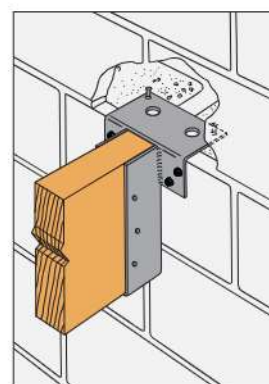
WMU Mid-Wall Installation See pp. 250–251 for models and information
