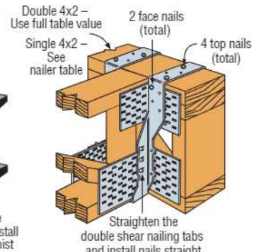
Typical THA422 Top Flange (Min.) Installation on a 4x2 Floor Truss
