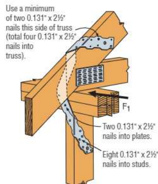
10 H7Z Installation
