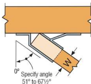
Top View U Hanger Skewed Right ≥ 51° (square cut)
