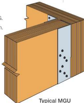
Typical MGU Installation with Right Flange Concealed
