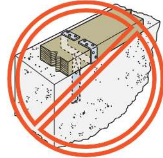
MAB Misinstallation (MAB straps must be separated before the concrete is poured or installed through 3/4"-diameter hole)
