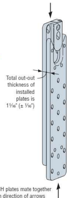
Assembly Thickness and Fit-Up Tolerance
