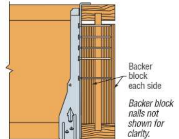
Face-Mount Hanger
