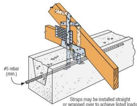
Typical DETAL Installation
