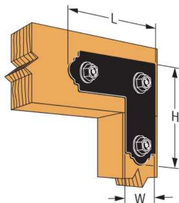
Typical APL4 Installation
