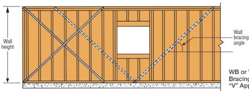
Typical RCWB Installation
