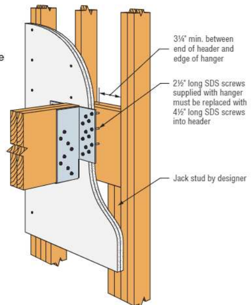
MGU Over Two Layers of 5/8" Drywall (LGU/HGU/HHGU similar)
