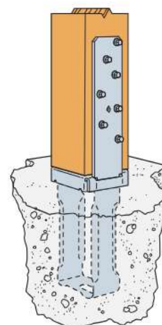
Figure 1 — Post Base with 1" Standoff
