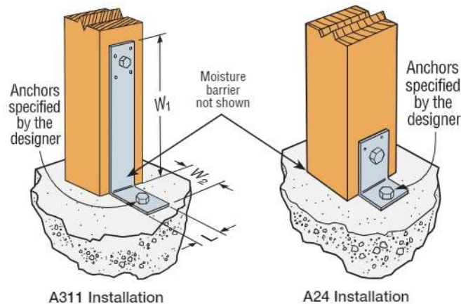
A311 Installation
