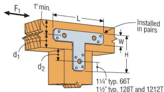
Typical T Installation
