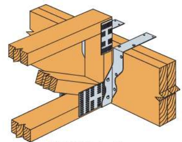
THA413 Top Flange (Max.) Installation
