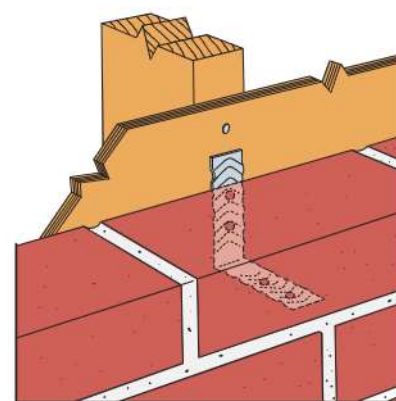
Typical BT Installation
