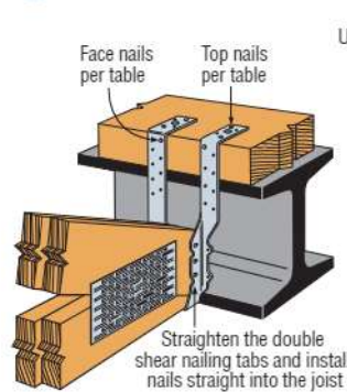
Typical THA Top Flange (Min.) Installation on a Nail (except THA29)
