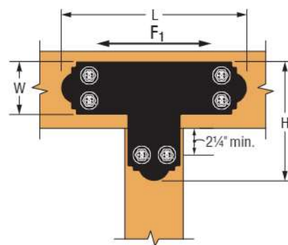
Typical APT6 Installation
