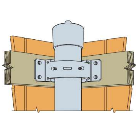
Typical PGTIC2Z-R Fence Installation
