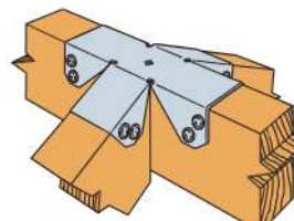
FWH2 Installation
