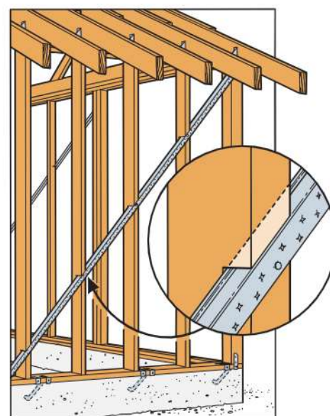
Typical RCWB Installation
