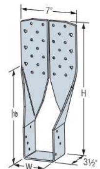
THGQ3.62-SDS (others similar)
