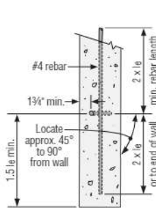
Midwall
