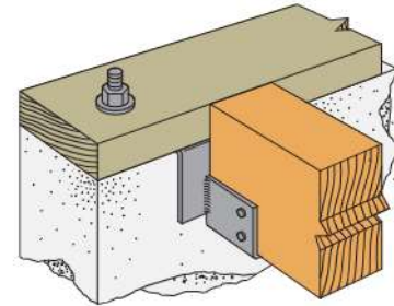
Typical GH Installation
