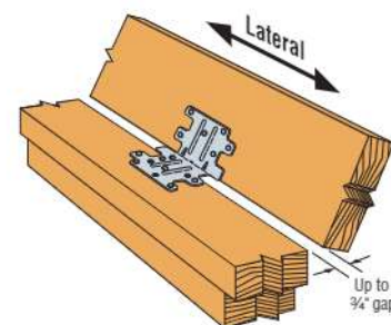
1 Typical RBC Installation (RBCP similar)
