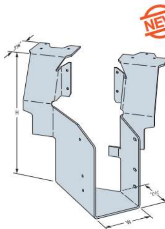
DGHT Skewed Right Shown (square-cut or bevel-cut joist allowed)
