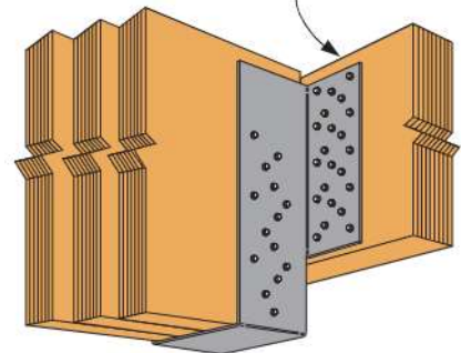
Typical HHGU Installation
