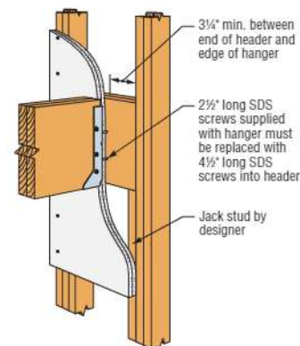
HUCQ Over Two Layers of 5/8" Drywall See engineering letter L-C-FACEMNTFW at strongtie.com for more information.
