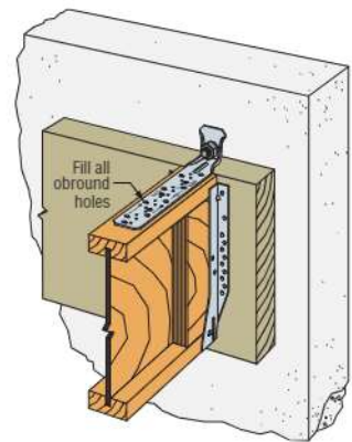
Typical LTPP2 Installation for I-joist
