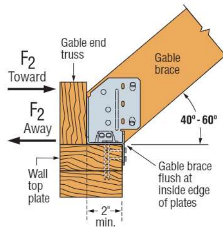
Typical Sloped Installation
