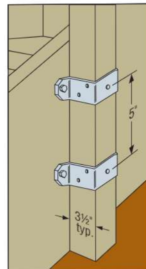
Typical DPT7Z Stairway Installation (DPT5Z similar)
