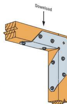
RTA2Z Installation
