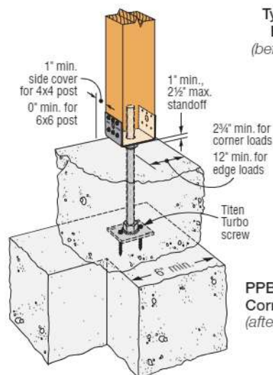
PPBF44 (PPBF66 similar)
