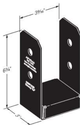
APVB44 (others similar)
