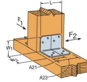
A21/A23 Installation
