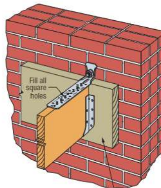
Typical LTPP2 Installation for Solid Sawn Joist
