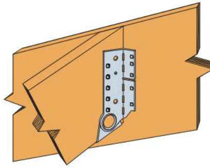
Typical LSSJ28LZ Installation with 2x10 Header (installation with 4x10 header similar)
