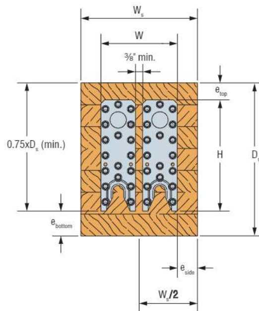
Double CBH on Carried Beam
