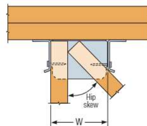
THJU26X Top View Installation
