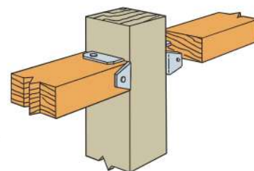
Typical FB24Z Installation
