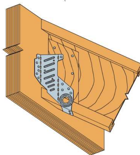
Typical LSSR Sloped Down and Skewed Right Installation (can be skewed left or right)
