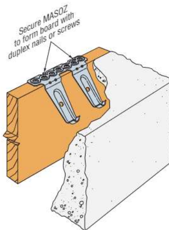
Typical MASOZ Installation in Concrete
