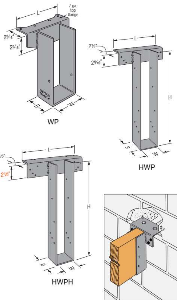
WMU Mid-Wall Installation See pp. 250–251 for models and more information.
