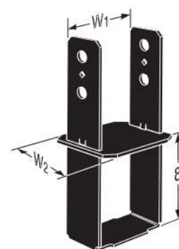
CBPC Classic (see pp. 80–81 for model no. and allowable loads)
