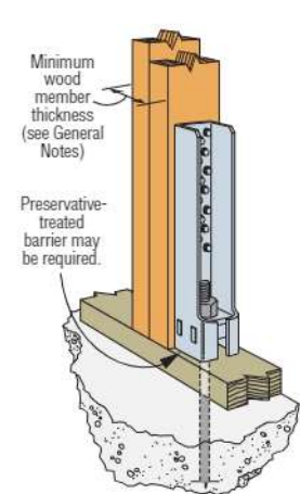
HDQ8 Vertical Installation
