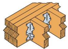
Ceiling Joists to Beam
