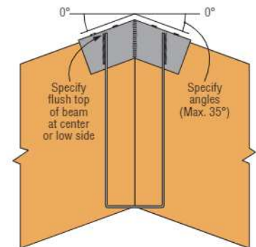
Typical WP Ridge Installation
