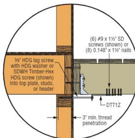
Typical DTT1Z Deck-to-House Lateral Load Connection
