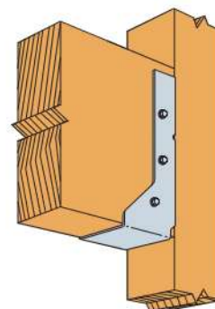
Typical HUCQ Installation on a Post
