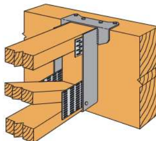
Typical WP Installation for 4x2 Truss
