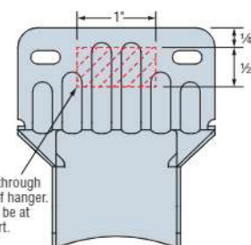
Panelized Installation Nailing Zone
