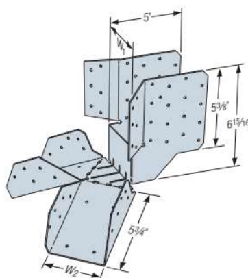
HHRC44 (others similar)
