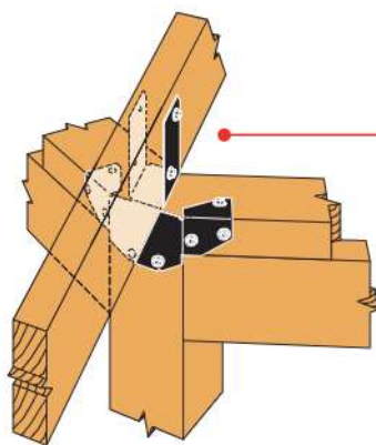
Typical APTG2 Installation
