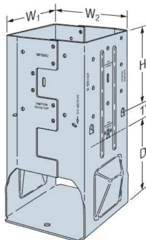
MPB88Z (MPB44Z, MPB66Z similar) US Patent 11,072,940
