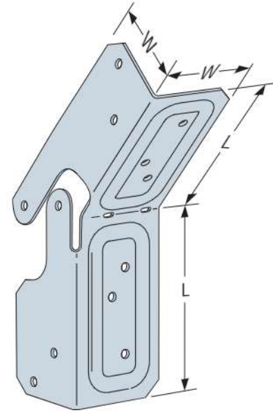
KBS1Z US Patent 9,045,895
