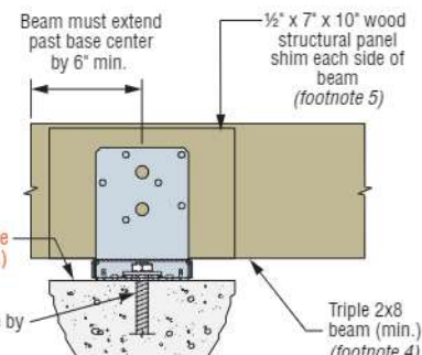
ABU66Z Beam Installation
