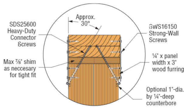
Top Connection for Back-to-Back Standard Installation
