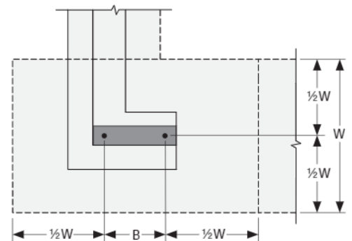
Footing Plan
