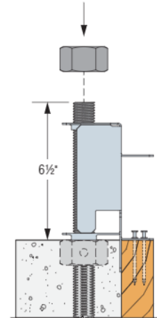
Anchor Bolt Height (Exterior)
