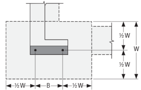
Footing Plan
