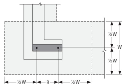
Footing Plan
