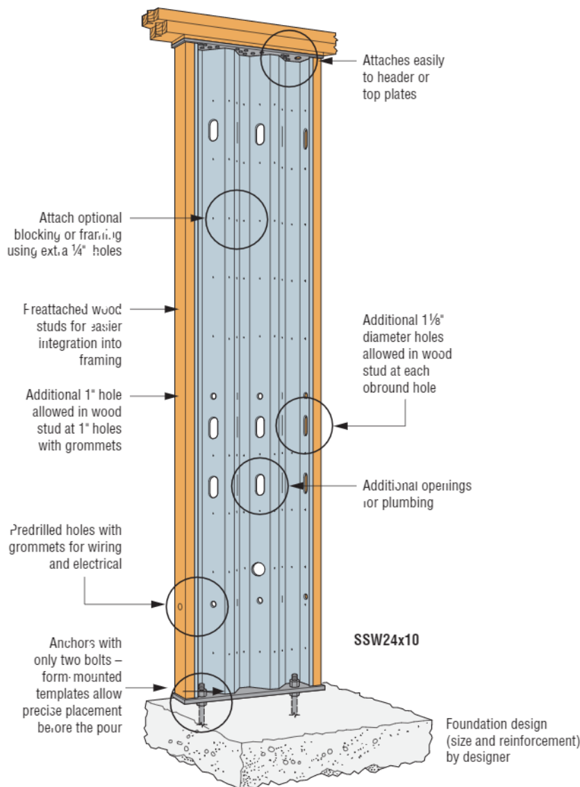
Standard Installation US Patent 8,281,551 Canadian Patent 2,489,845
