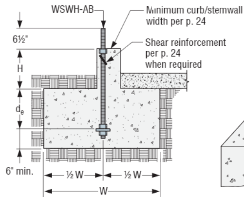
Curb or Stemwall Section View
