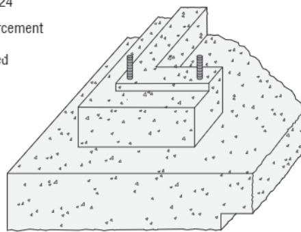
Perspective View
