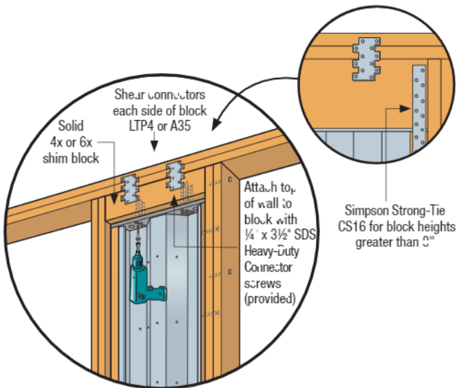
Top-of-Wall Connection
