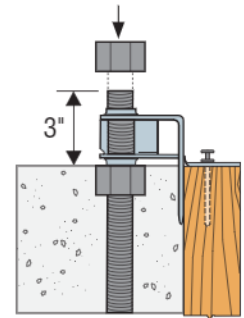
Anchor Bolt Height (Exterior)
