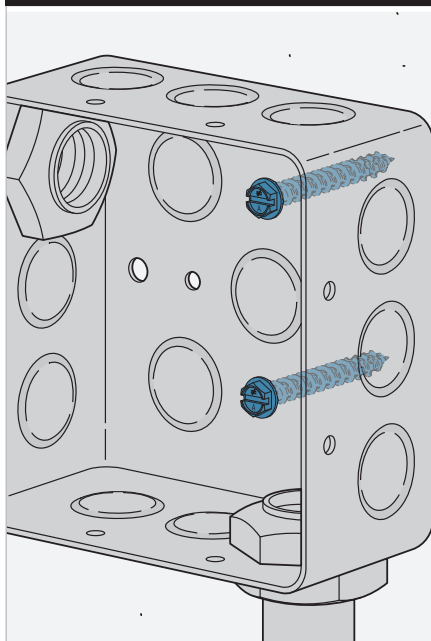
Titen Turbo™ Concrete and Masonry Screw Anchor (Hex-Head)
