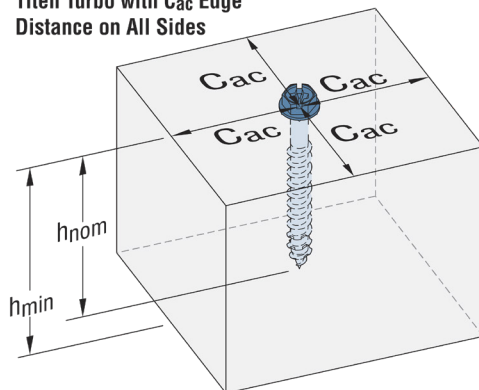
Flat Slab
