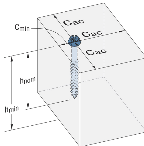
Titen Turbo with c_{min} Edge Distance on One Side and c_{ac} on Three Sides
