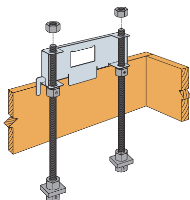
WSWH-RT Exterior Installation* US Patent 7,445,192
