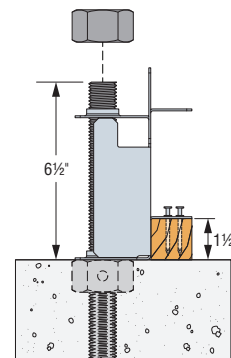
Anchor Bolt Height (Interior)
