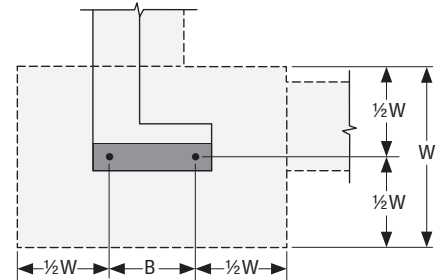
Footing Plan
