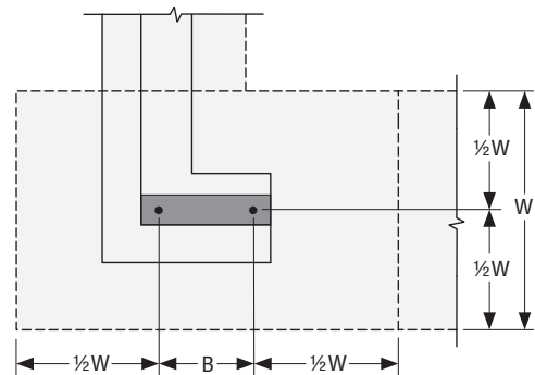
Footing Plan
