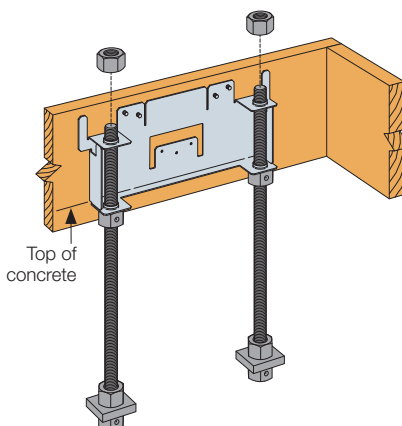
WSWH-RTPF (Panel form) US Patent 7,445,192
