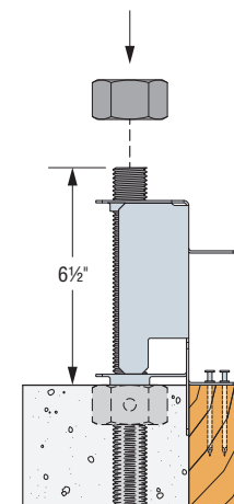
Anchor Bolt Height (Exterior)
