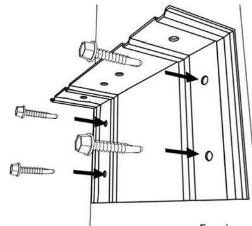
Framing Member
