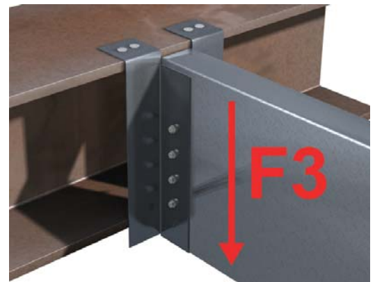
Load Direction
