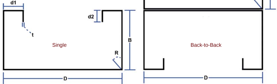
Single & Back-to-Back StiffWall® Column Product Profile
