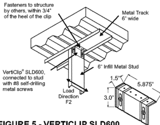
FIGURE 5 - VERTICLIP SLD600
