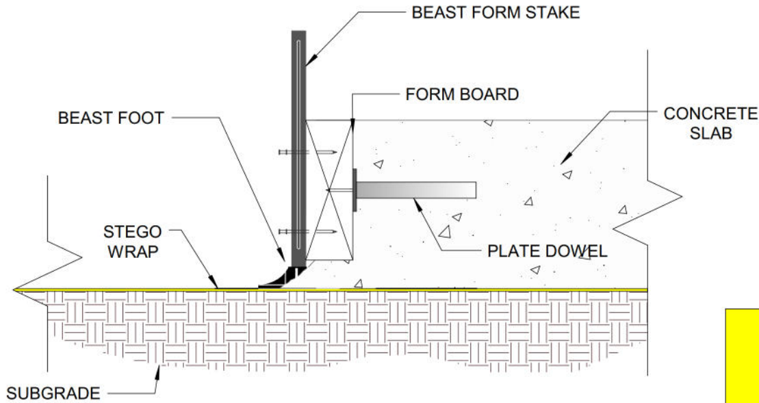
PROFILE VIEW
